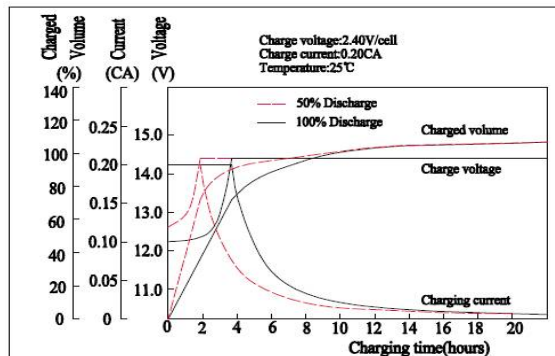
Charging Characteristics(25°C)
