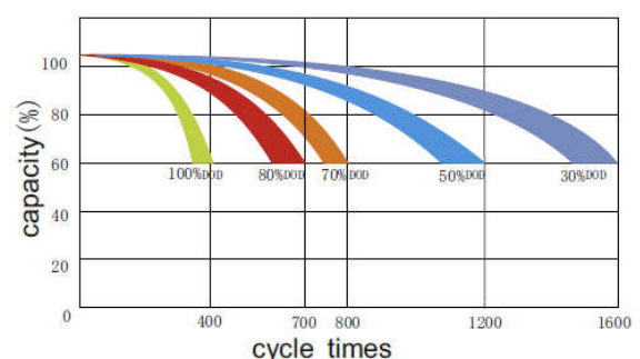
Cycle life Vs discharge depth
