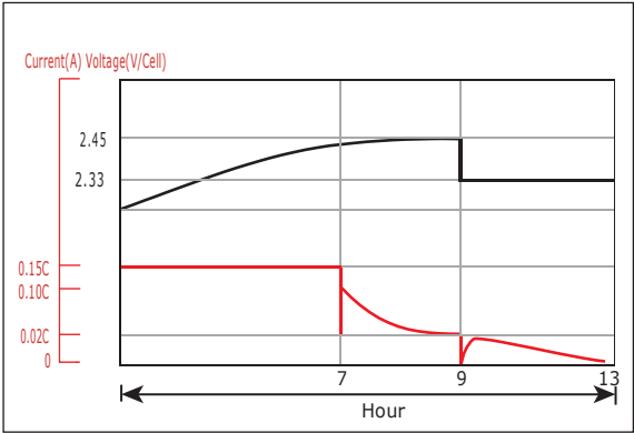
Charge performance
