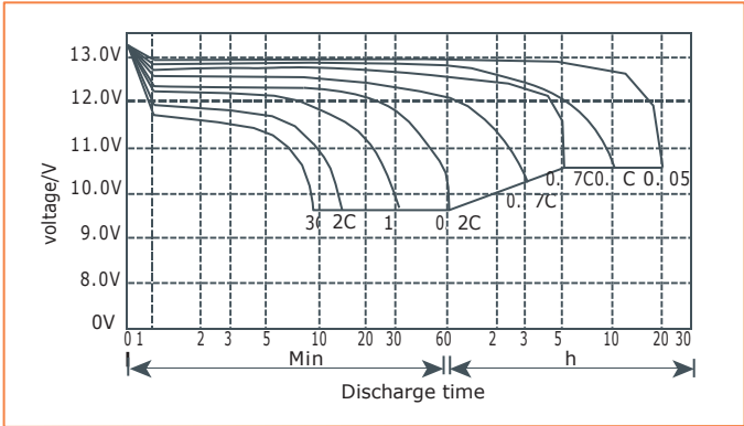
Discharge performance
