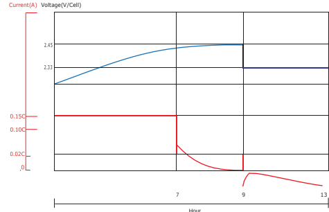
Charge performance
