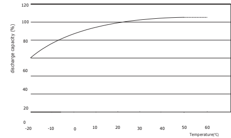
Discharge capacity vs. temperature
