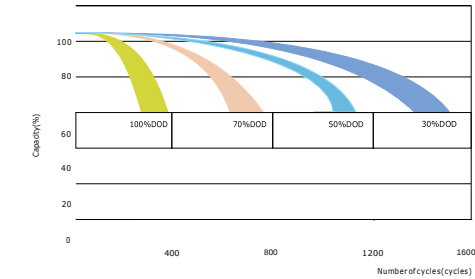
Cycles vs. discharge depth
