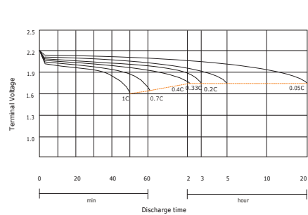
Discharging performance
