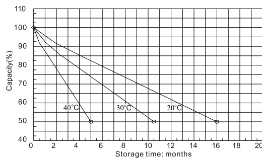
Self-discharge characteristic
