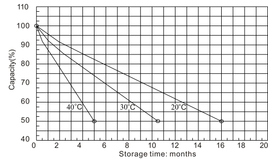
Self-discharge characteristic
